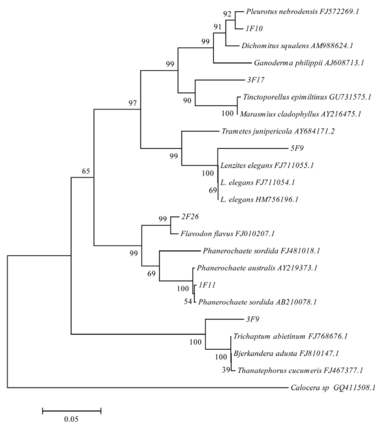
Figure 3. Phylogenetic relationships of endophytic fungi isolated from Vitis labrusca belonging to Basidiomycota phylum; the isolates belonged to Orders: Agaricales (Families: Schizophyllaceae and Pleurotaceae); Corticiales (Families: Corticiaceae); Polyporales (Family: Corioliaceae and Genus Flavodon , Incertae sedis Family); Russulales (Family: Meruliaceae). The sequence analysis was based on partial ITS1-5.8S-ITS2 rRNA sequences obtained from endophytes and closely related sequences that are based on a distance analysis (neighbor-joining algorithm with the Jukes-Cantor model; 1000 bootstrap replicates performed).
