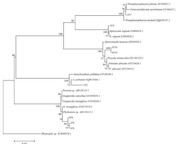
Figure 2. Phylogenetic relationships of endophytic fungi isolated from Vitis labrusca belonging to Ascomycota phylum; the isolates belonged to Class Dothideomycetes (Families: Botryosphaeriaceae, Dothioraceae, Montagnulaceae, Sporormiaceae and Genus Epicoccum , Aporospora , both Incertae sedis Family). The sequence analysis was based on partial ITS1-5.8S-ITS2 rRNA sequences obtained from endophytes and closely related sequences that are based on a distance analysis (neighbor-joining algorithm with the Jukes-Cantor model; 1000 bootstrap replicates performed).
