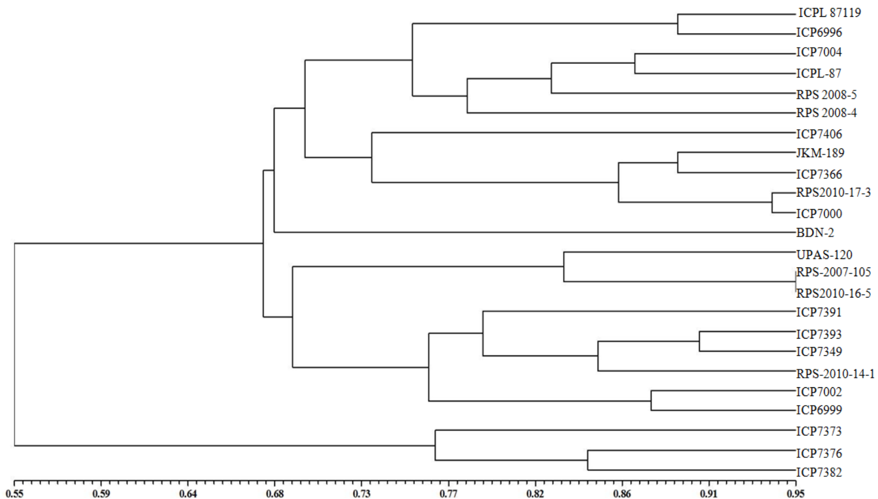
Fig-2: Dendrogram constructed using UPGMA based on Jaccard's coefficient of 24 pigeonpea genotypes (SSR Markers)
