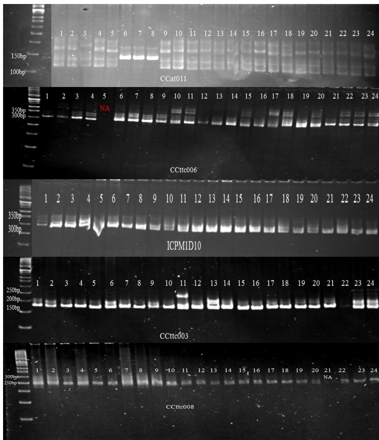
Fig 1. SSR Profile generated by ICPM1H01, ICPM2B08, ICPM1E04 (not amplified), CCac036, CCttc033, CCat011, CCttc006, ICPM1D10, CCttc003 and CCttc008 (10) primer of 24 pigeonpea germplasm including varieties.
