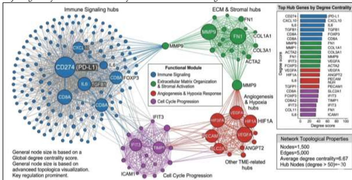
Fig 3. Protein–Gene Interaction Network and Hub Biomarkers in TME.
