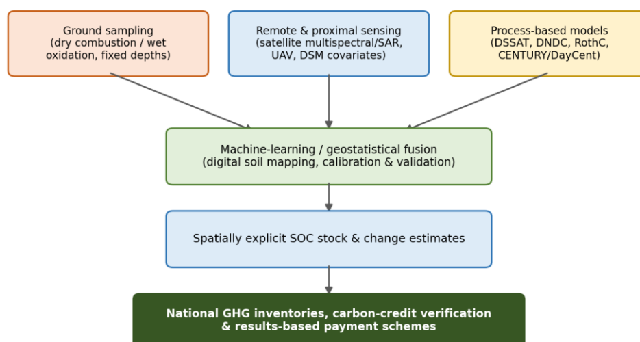
Figure 4. Integrated measurement-monitoring-reporting-verification (MMRV) framework combining ground sampling, remote/proximal sensing, and process-based modelling to support national GHG inventories and carbon-credit verification.
