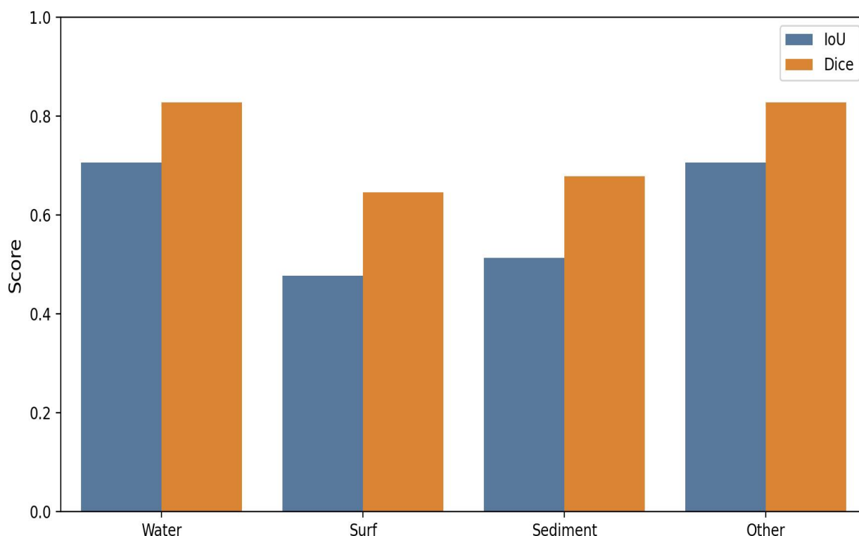
Figure 1. Per-class segmentation performance measured using Intersection over Union (IoU) and Dice coefficient.
