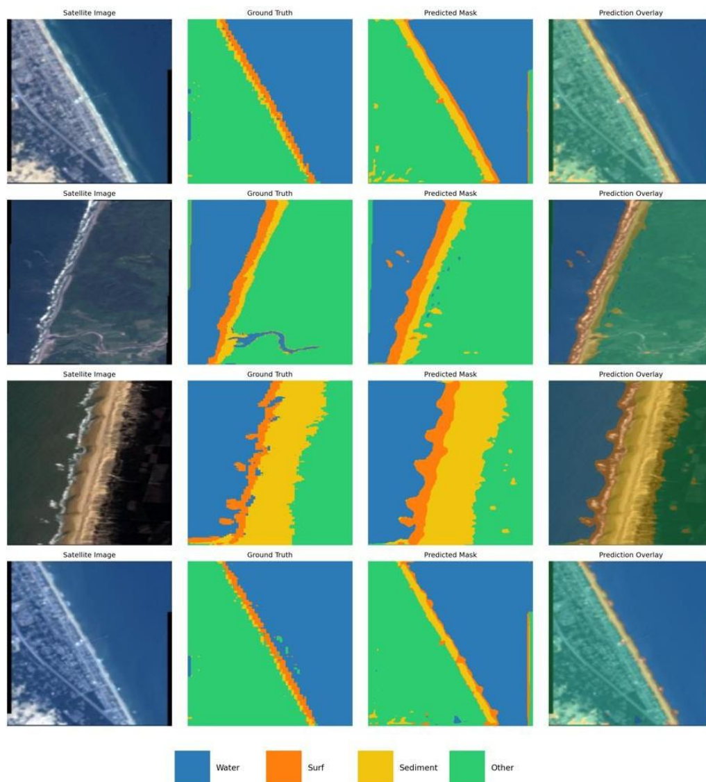
Figure 3. Sample Segmentation Results
