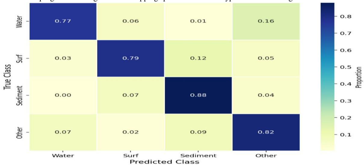
Figure 2. Normalized Confusion Matrix
