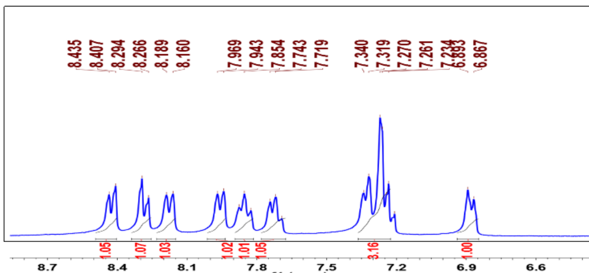
Fig. 4 ^1\text{H} NMR (300MHz, \text{CDCl}_3 ) expansion of QCAP
