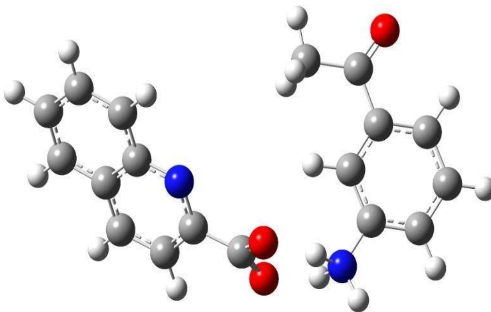
Fig. 8 Optimized structure of QCAP
