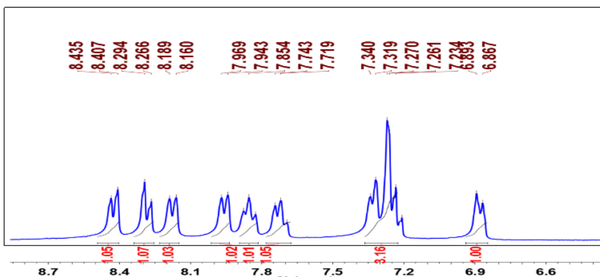
Fig. 3 ^1\text{H} NMR (300MHz, \text{CDCl}_3 ) expansion of QCAP
