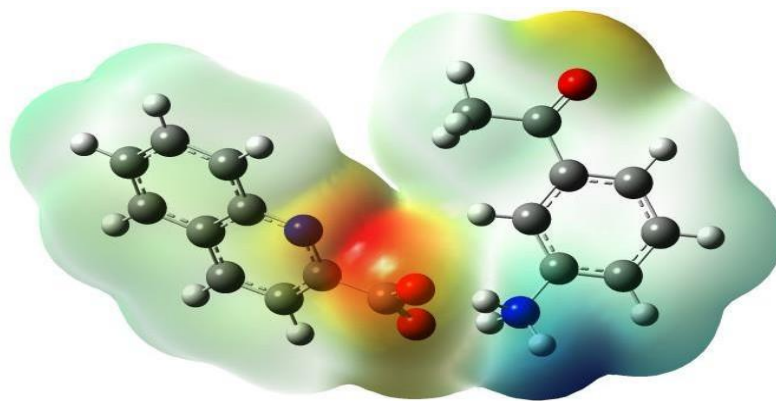
Fig. 9 Molecular Electrostatic Potential of QCAP
