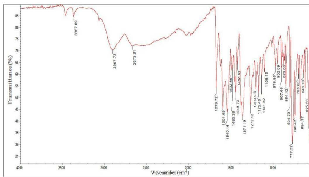
Fig. 5 FT-IR spectrum of QCAP
