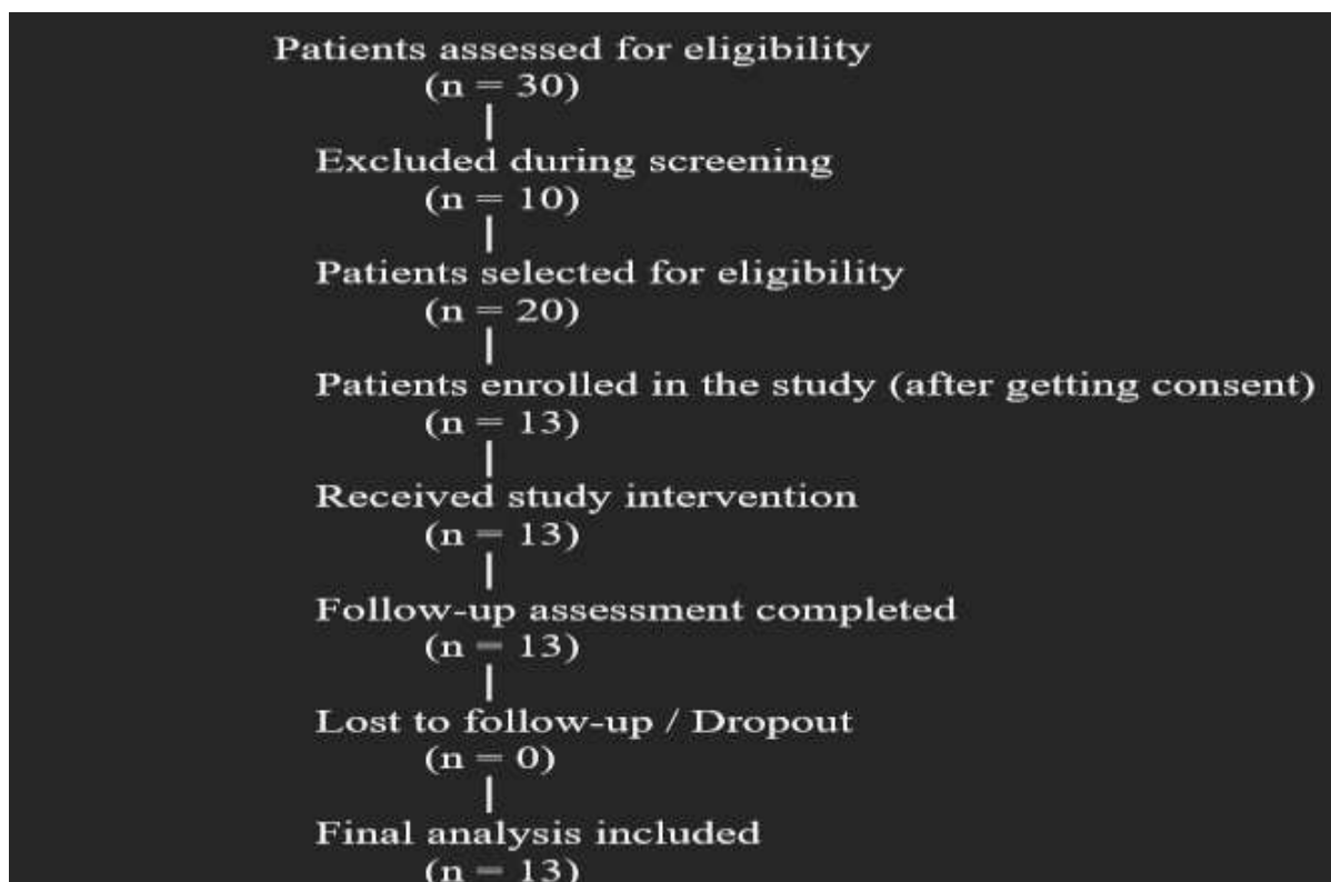
Fig.1 Flow Chart
