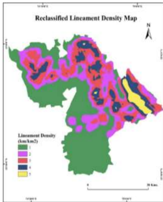
Fig. 4. Reclassified map of Lineament Density.
