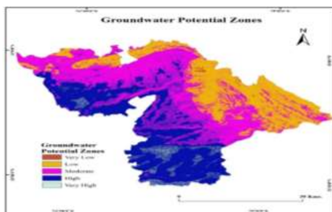
Fig. 10. Groundwater potential zone map of Jammu district.
