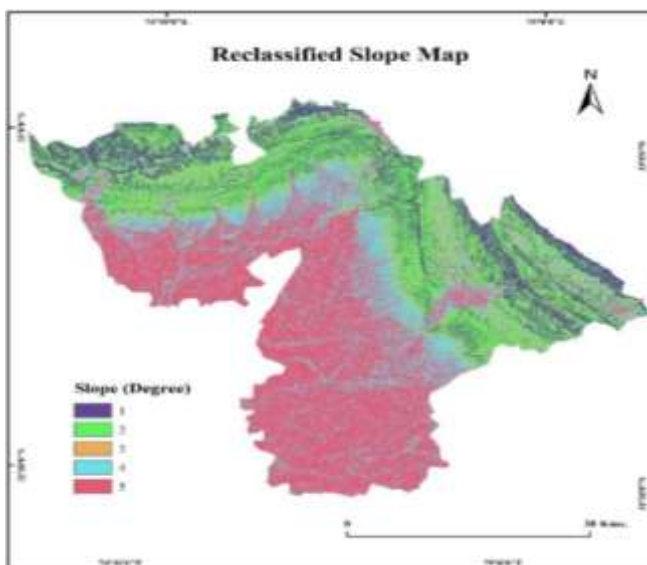
Fig. 6. Reclassified map of Slope.
