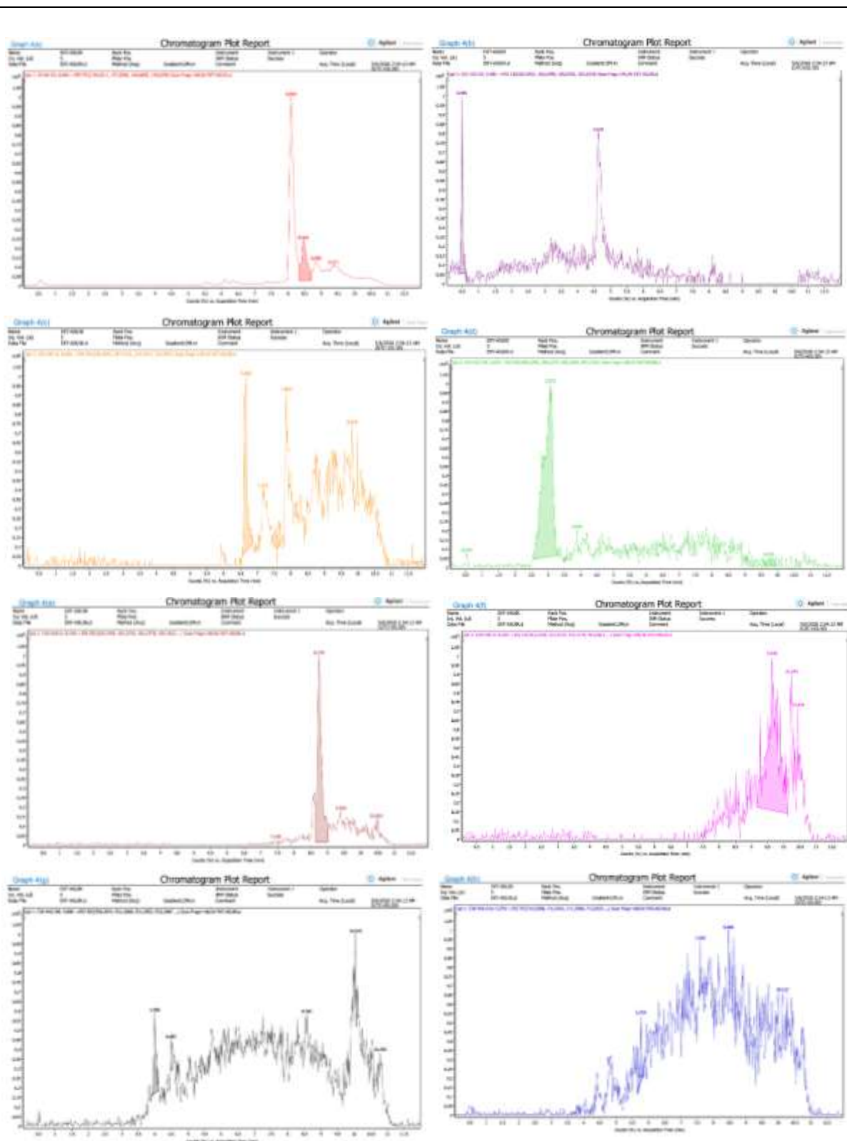
Figure 12 a : LC–MS chromatographic profile of the hydroethanolic extract of Urginea indica Kunth indicating the retention times of the detected C_6H_6O_3 compound.
