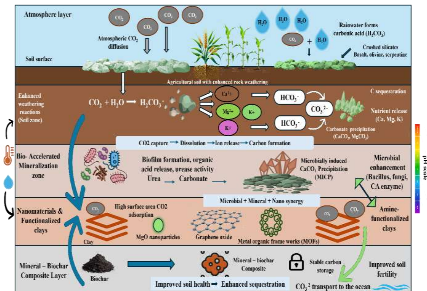
Figure 4. Enhanced rock weathering system integrating minerals, microbial processes, biochar and nanomaterials for CO 2 capture and soil carbon stabilization.
