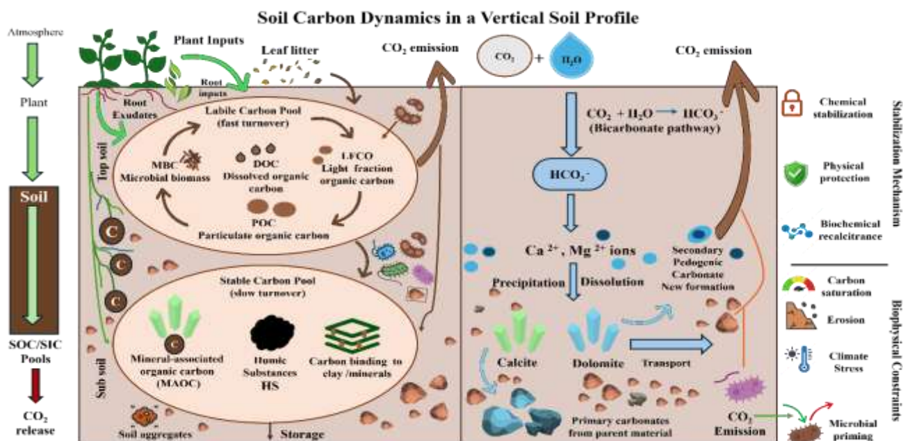
Figure 2. Vertical soil profile illustrating organic and inorganic carbon cycling, stabilization mechanisms, and CO 2 fluxes between soil and the atmosphere
