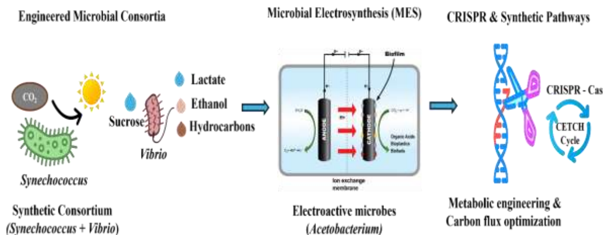
Figure 3. Engineered biological strategies for carbon stabilization, including microbial consortia, microbial electrosynthesis, and CRISPR-based metabolic engineering.
