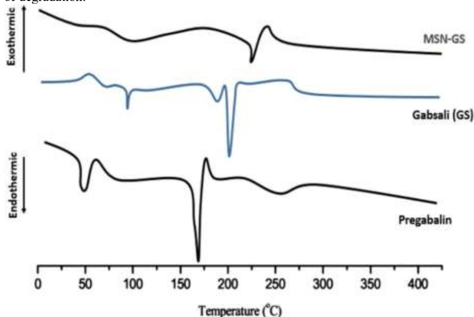
Figure 2: Differential scanning calorimetry (DSC) thermograms of pure pregabalin and optimized microsphere formulation.
