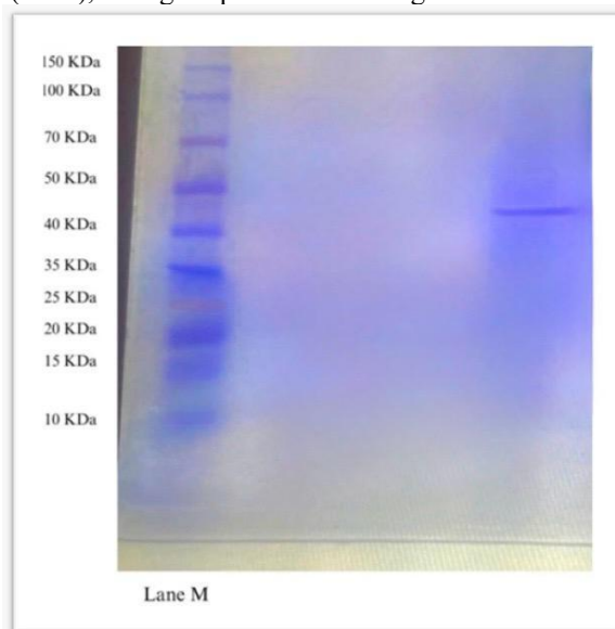
Fig. 10 SDS-PAGE protein Electrophoresis and determination of molecular weight of lipase from Aspergillus flavus RRF2-MH279408
