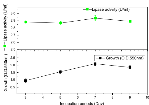
Fig. 4 Effect of incubation days on growth and lipase production by Aspergillus flavus RRF2- MH279408
