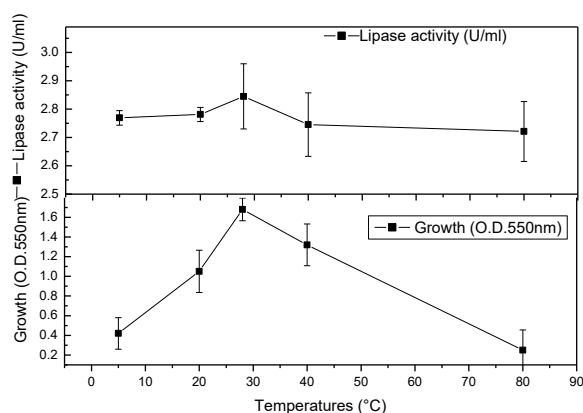
Fig.8 Effect of different temperatures on growth and lipase production by Aspergillus flavus RRF2-MH279408
