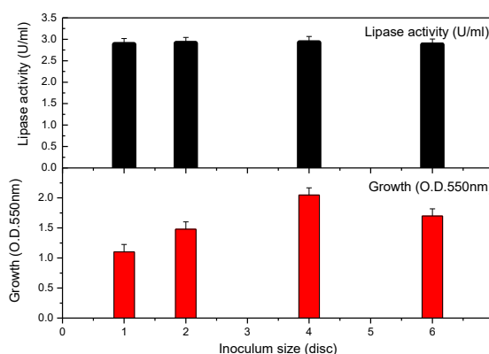
Fig. 9 Effect of inoculum sizes on growth and lipase production Effect of different carbon sources on growth and lipase production by Aspergillus flavus RRF2- MH279408
