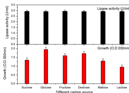
Fig. 5 Effect of different carbon sources on growth and lipase production Aspergillus flavus RRF2- MH279408
