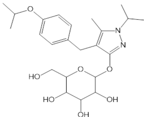
Fig 3: Remogliflozin
