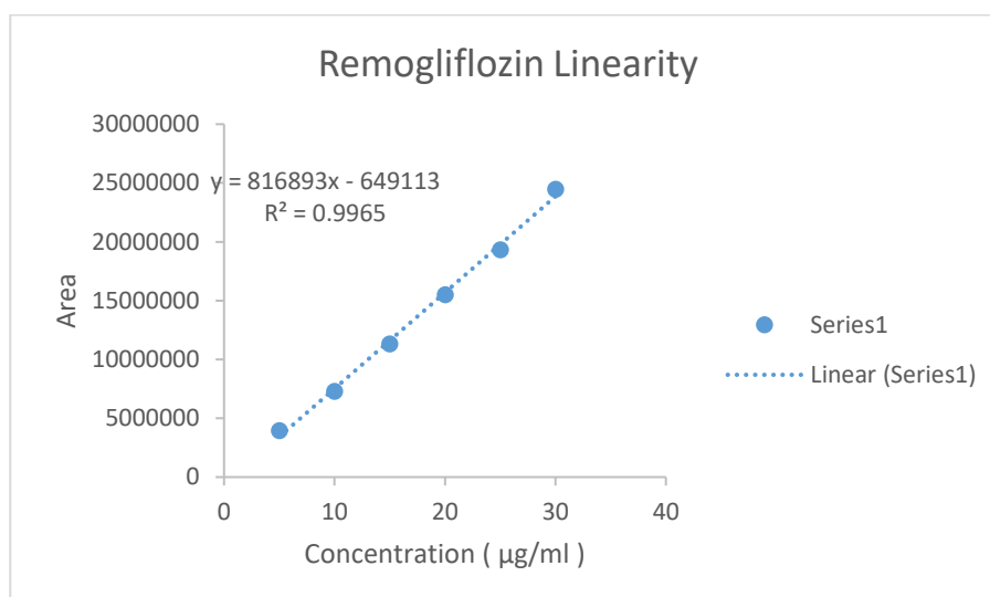
Fig 7: Graph for linearity studies
