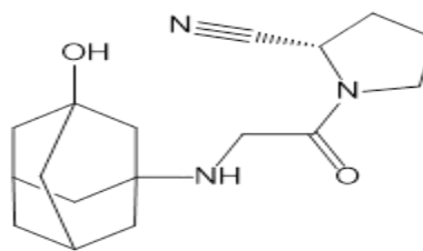
Fig 2: Vildagliptin
