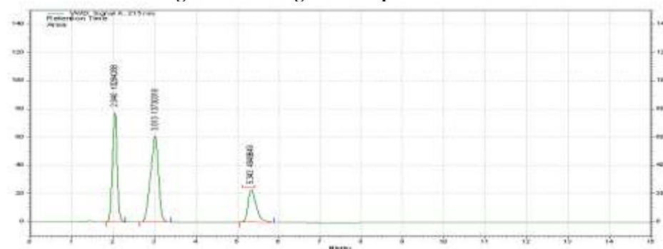
Fig 5: Chromatogram for optimised method
