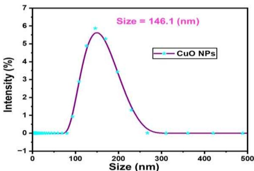
Fig. 6. DLS particles size analysis of CuO NPs
