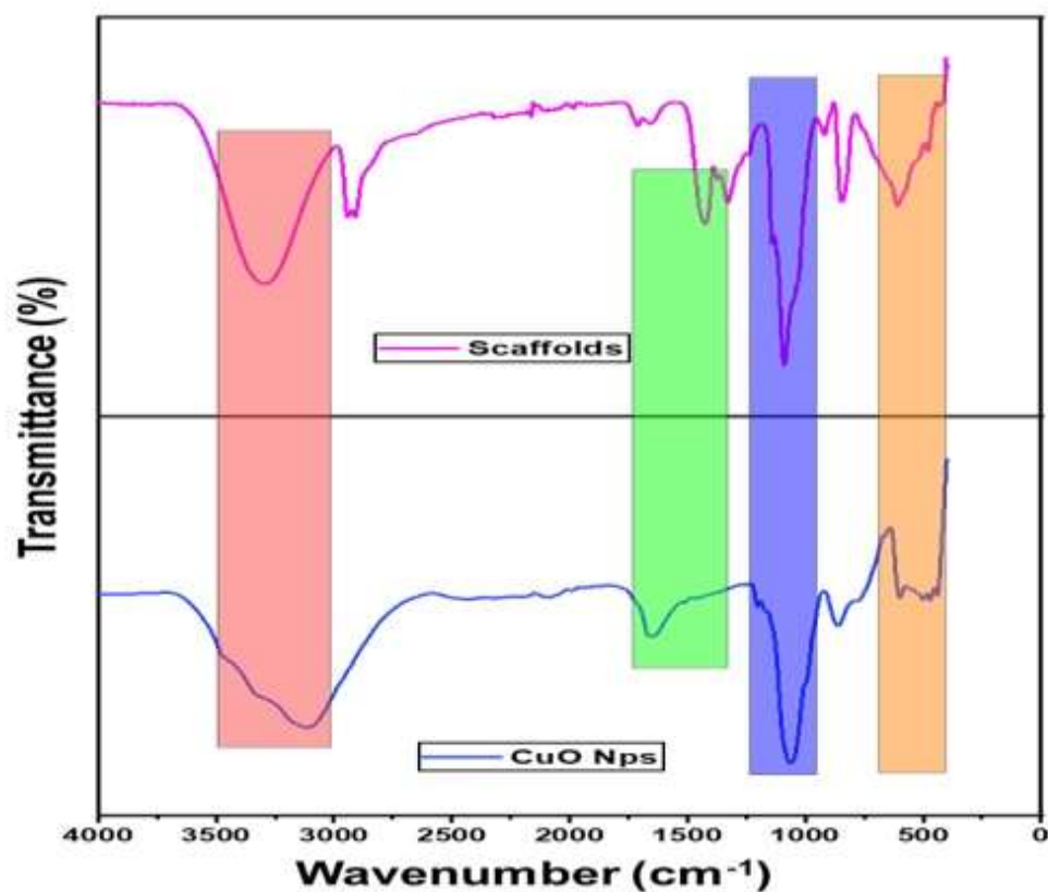
Fig. 2. FTIR spectra of CuO NPs and their incorporation into nanoscaffolds.
