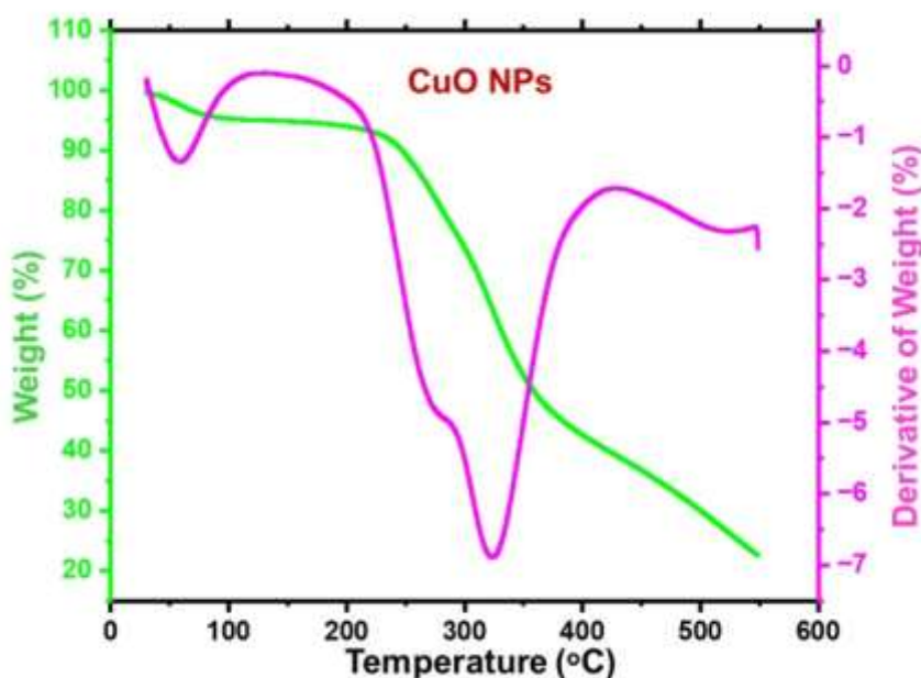
Fig. 5. Thermal degradation behavior of CuO-incorporated nanoscaffolds
