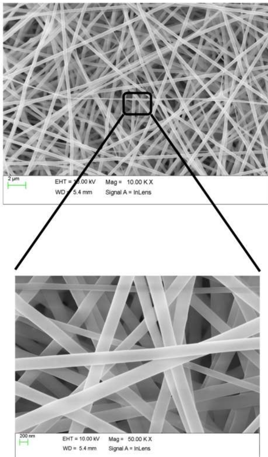
Fig. 4. SEM analysis of starch/PVA/CuONPs nanoscaffolds
