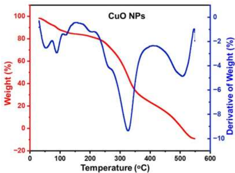
Fig. 5. TGA analysis of starch/PVA/CuONPs nanoscaffolds
