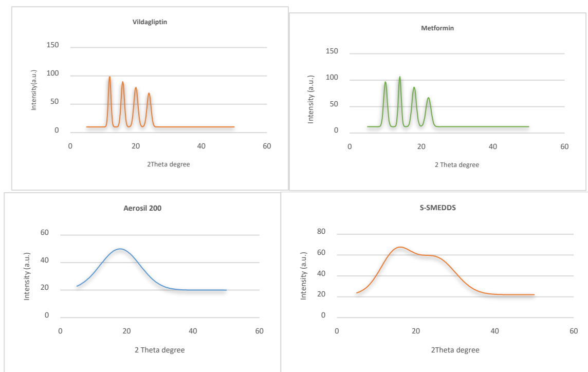
Figure 3. (a) XRD of Pure API vildagliptin, (b) Metformin HCl, (c) Aerosil 200, (d) Powder SMEDDS.
