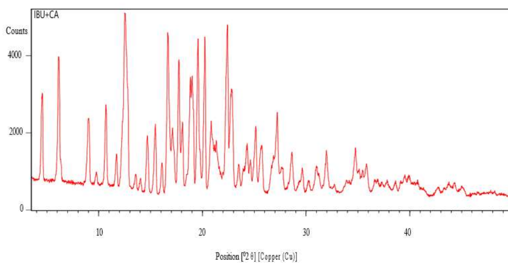
Figure 15: XRD spectrum of physical mixture (IBU+CA)
